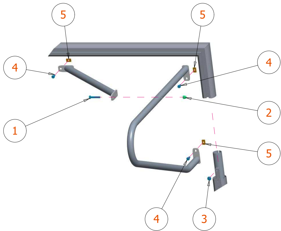
DETAIL A
